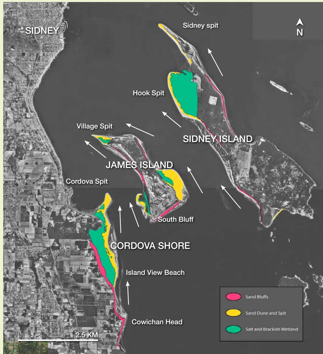
FIGURE 2. SAND BLUFFS, DUNES, SPITS, AND COASTAL WETLANDS IN THE CORDOVA SHORE-JAMES ISLAND-SIDNEY ISLAND AREA OF SOUTHERN STRAIT OF GEORGIA. Feeder bluffs are shown in red, coastal sand ecosystems are shown in yellow, and coastal wetlands are shown in green. The prevailing direction of sediment transport is shown with white arrows (from the south and southeast).
